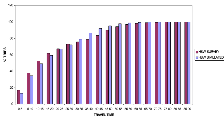
FIGURE 4.5.1- CUMULATIVE TRIP LENGTH FREQUENCIES FOR HBW
