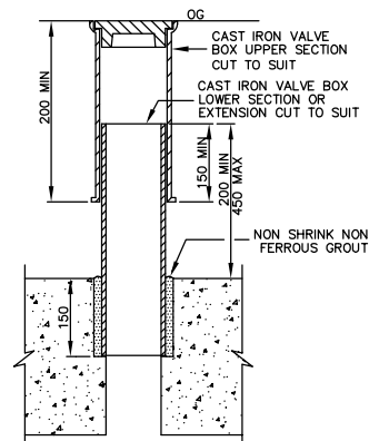
VALVE BOX DETAIL
